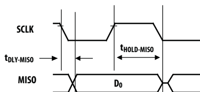
MOSI delay and hold time during read operation
